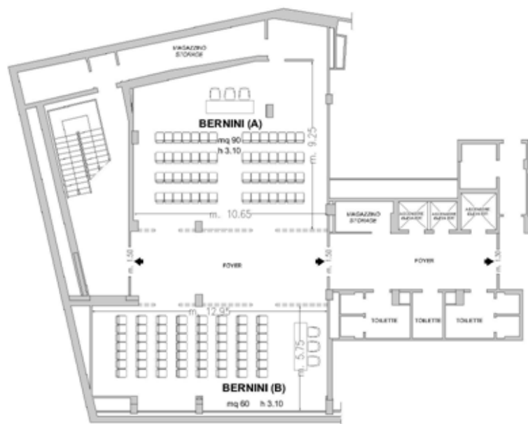
Piano -1 / Basement
