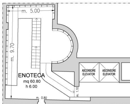
Piano -1 / 1st Basement
